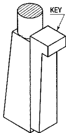
Lewis bolt FIG. 24-68
