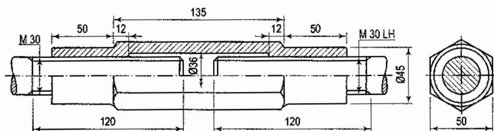
Coupler-nut FIG. 23-24
