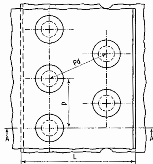
Double-riveted (zigzag) lap joint
