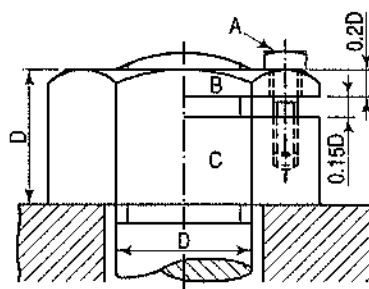
Sawn nut
