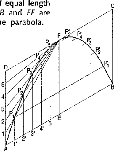
Parallelogram method
